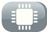
Fuzzy Logic
